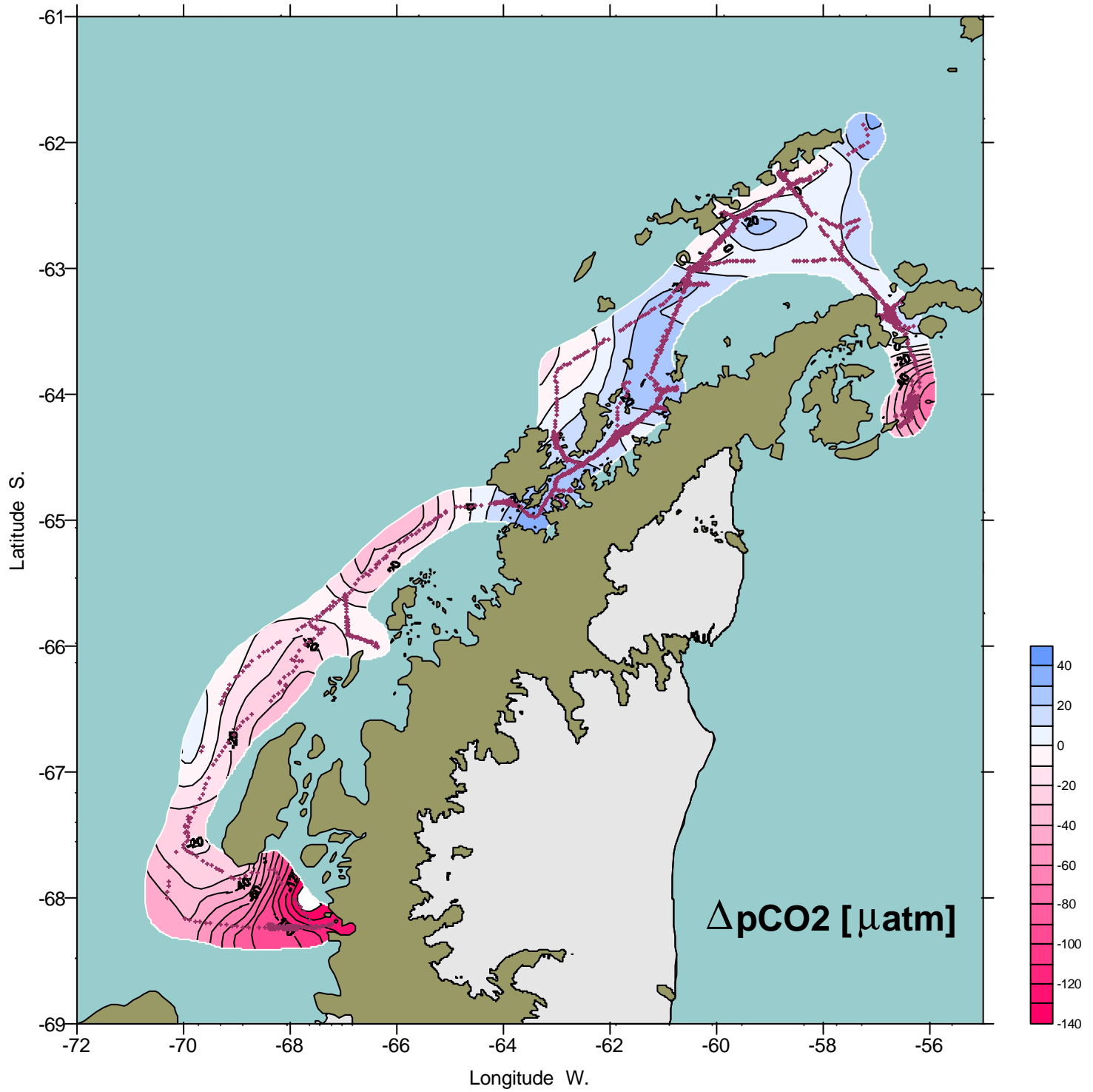
Distribution of \Delta p\text{CO}_2 between sea-surface and air (April 2000)
