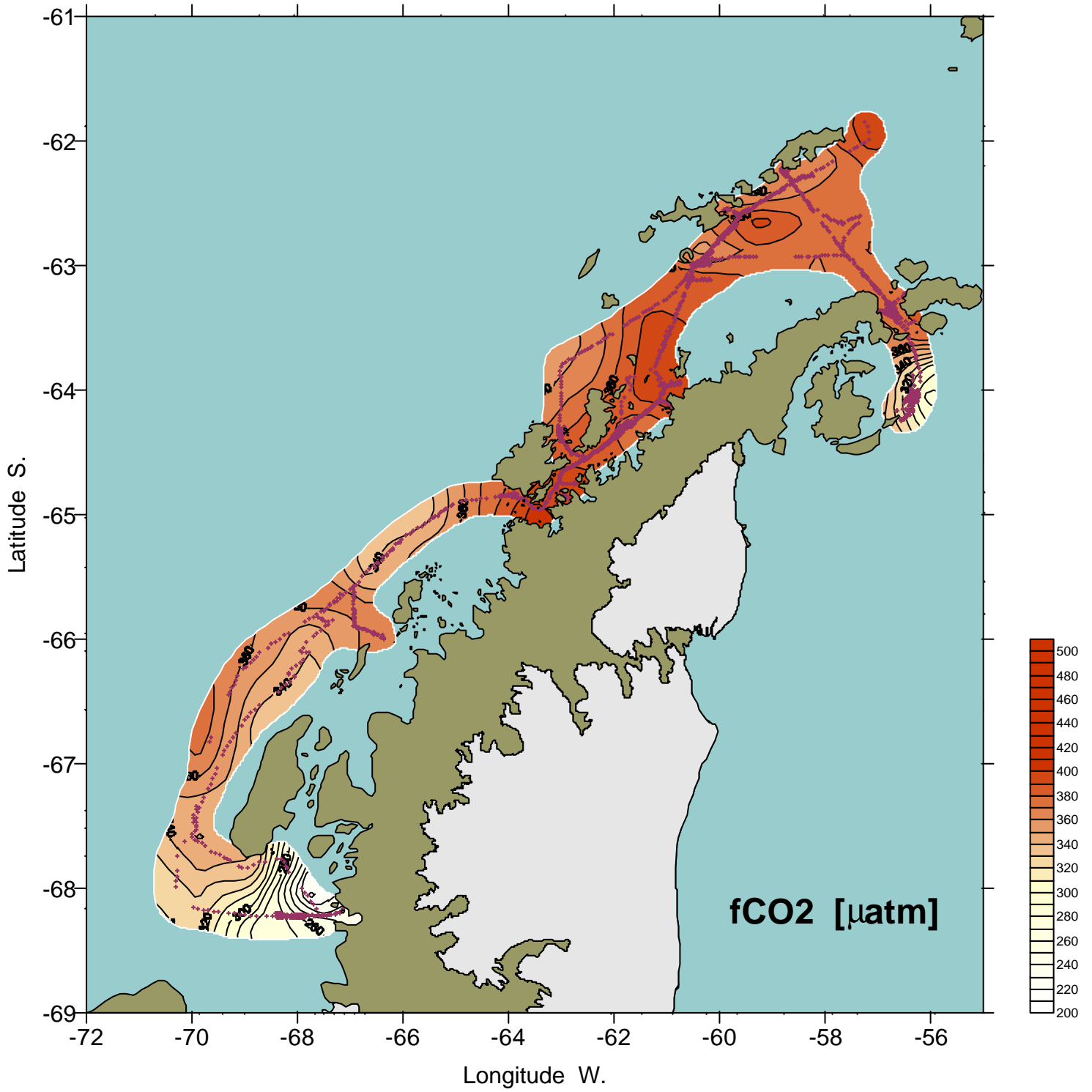
Sea-surface distribution of CO 2 in water (April 2000)
