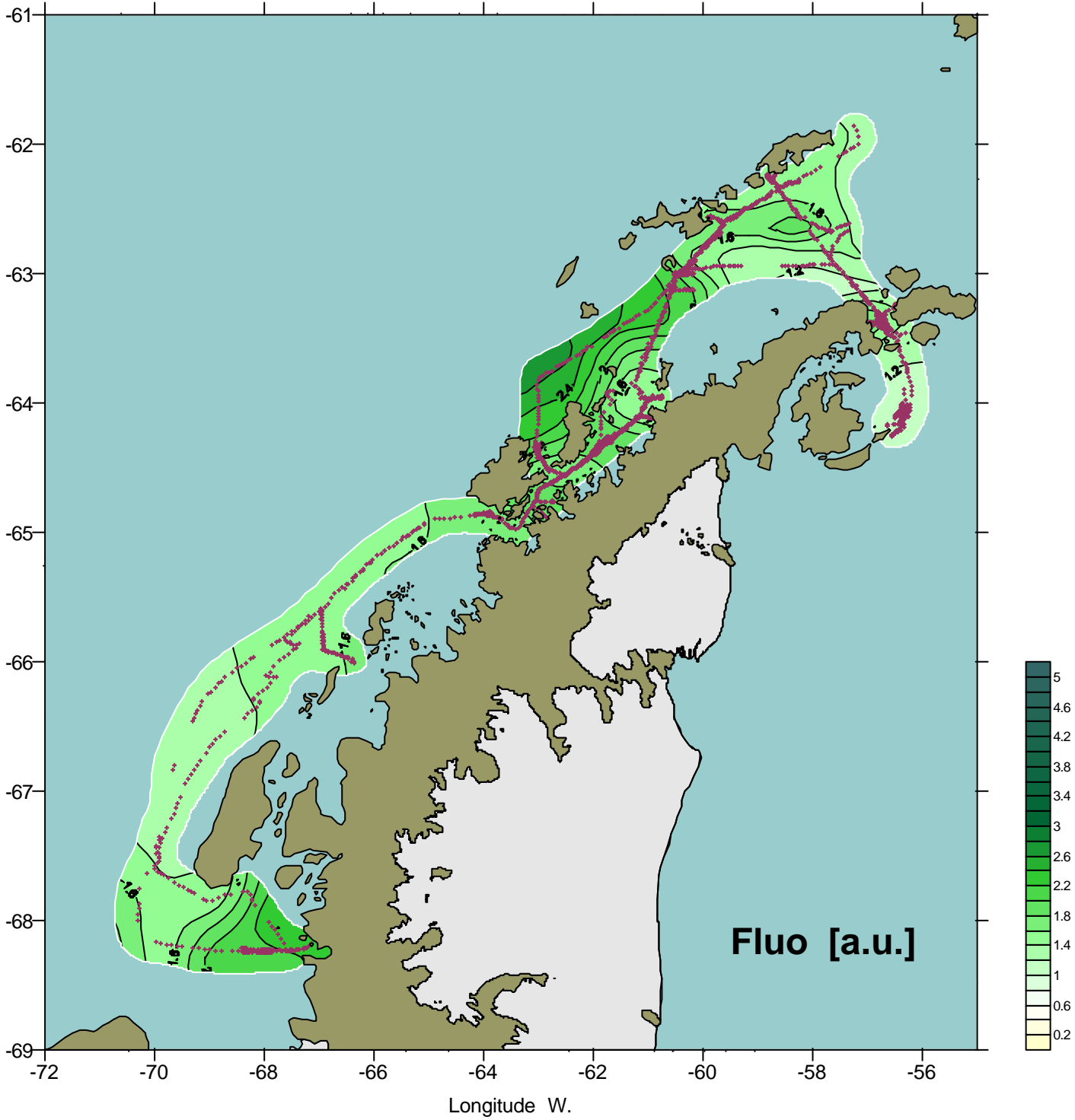
Sea-surface fluorescence distribution (April 2000)
