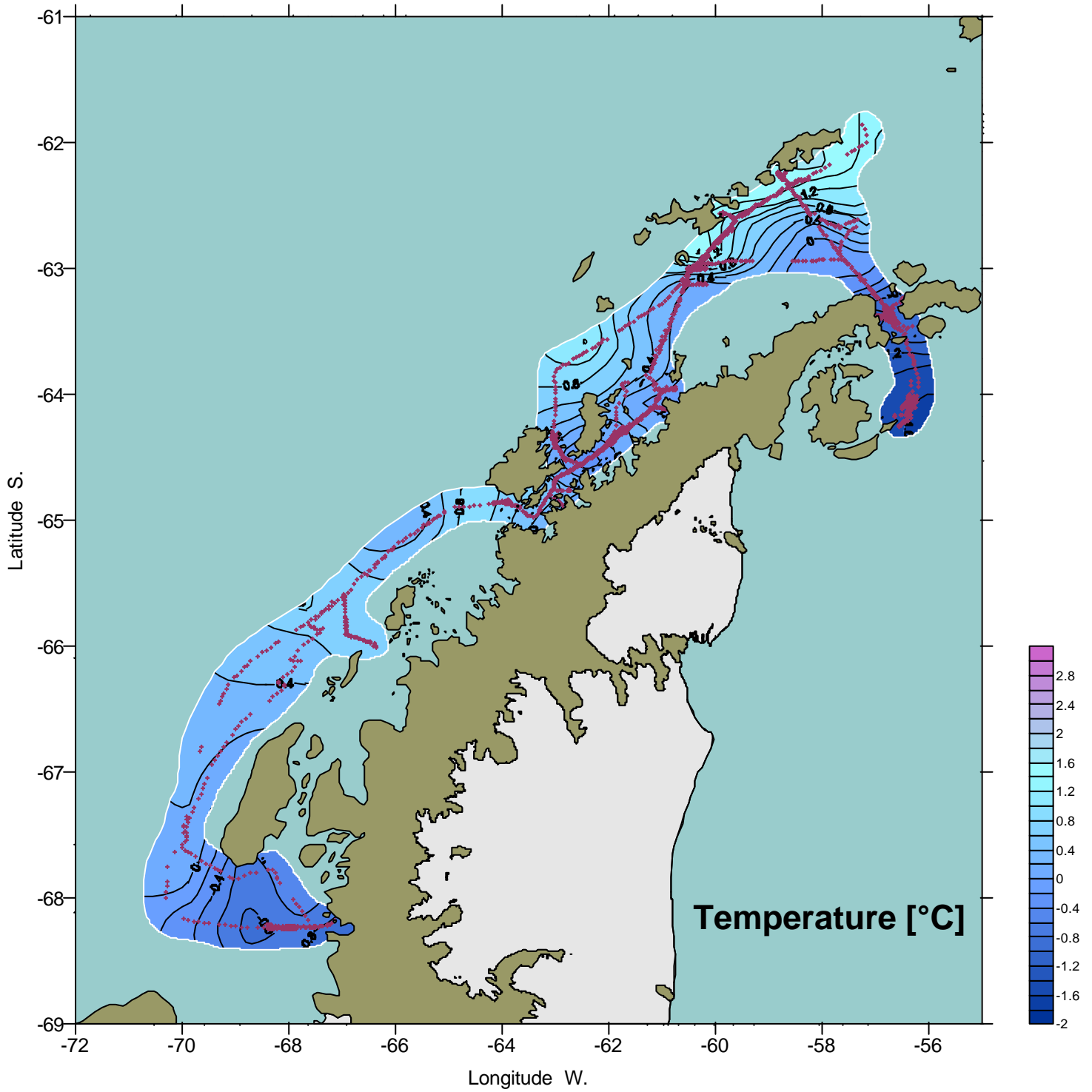
Sea-surface temperature distribution (April 2000)
