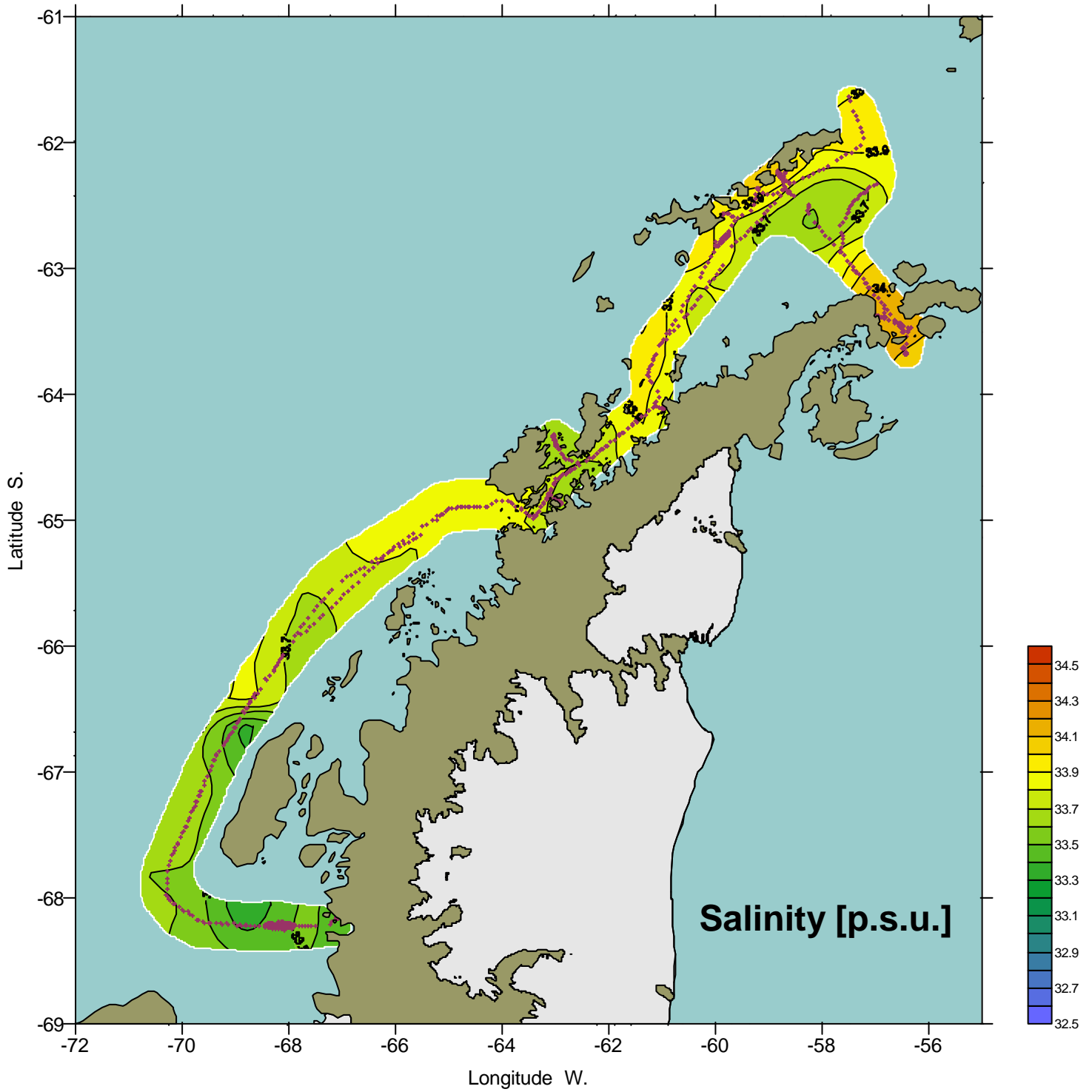
Sea-surface salinity distribution (March 2001)
