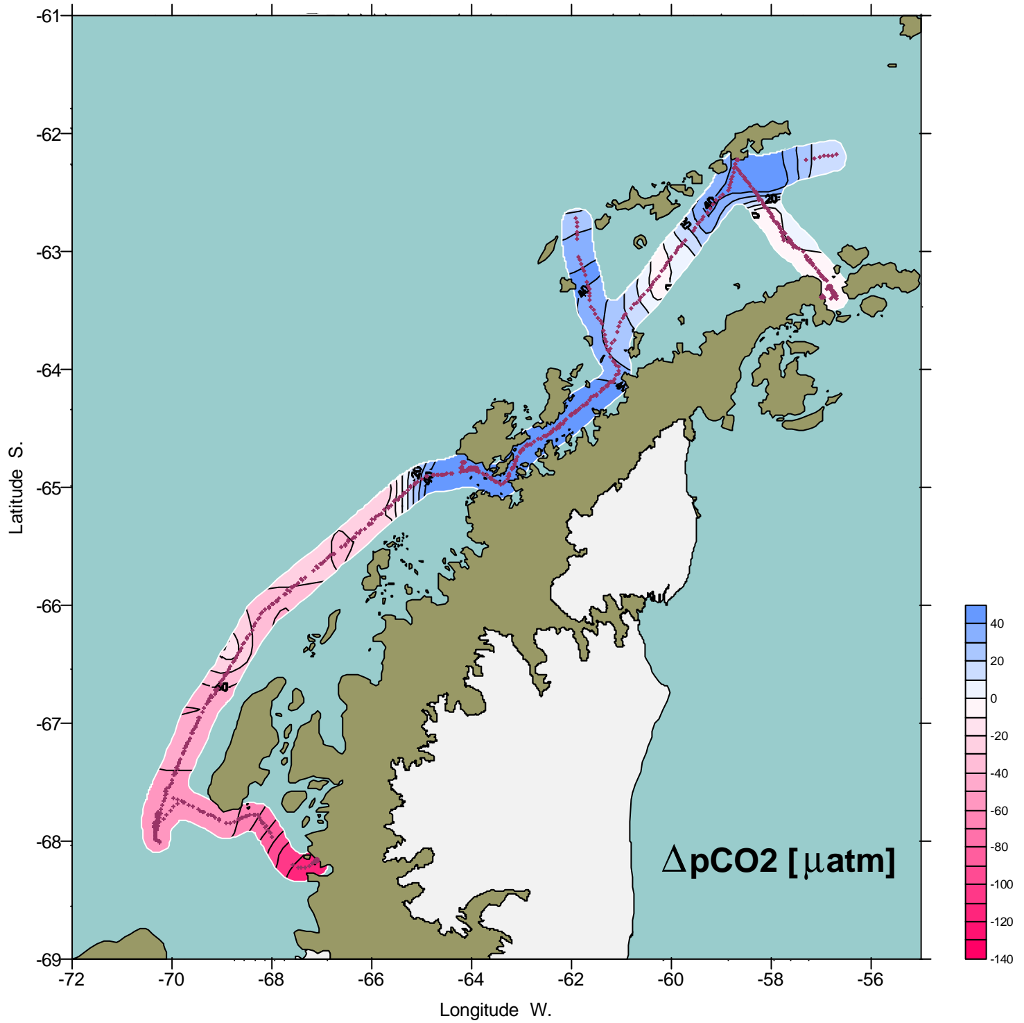
Distribution of \Delta p\text{CO}_2 between sea-surface and air (April 2002)
