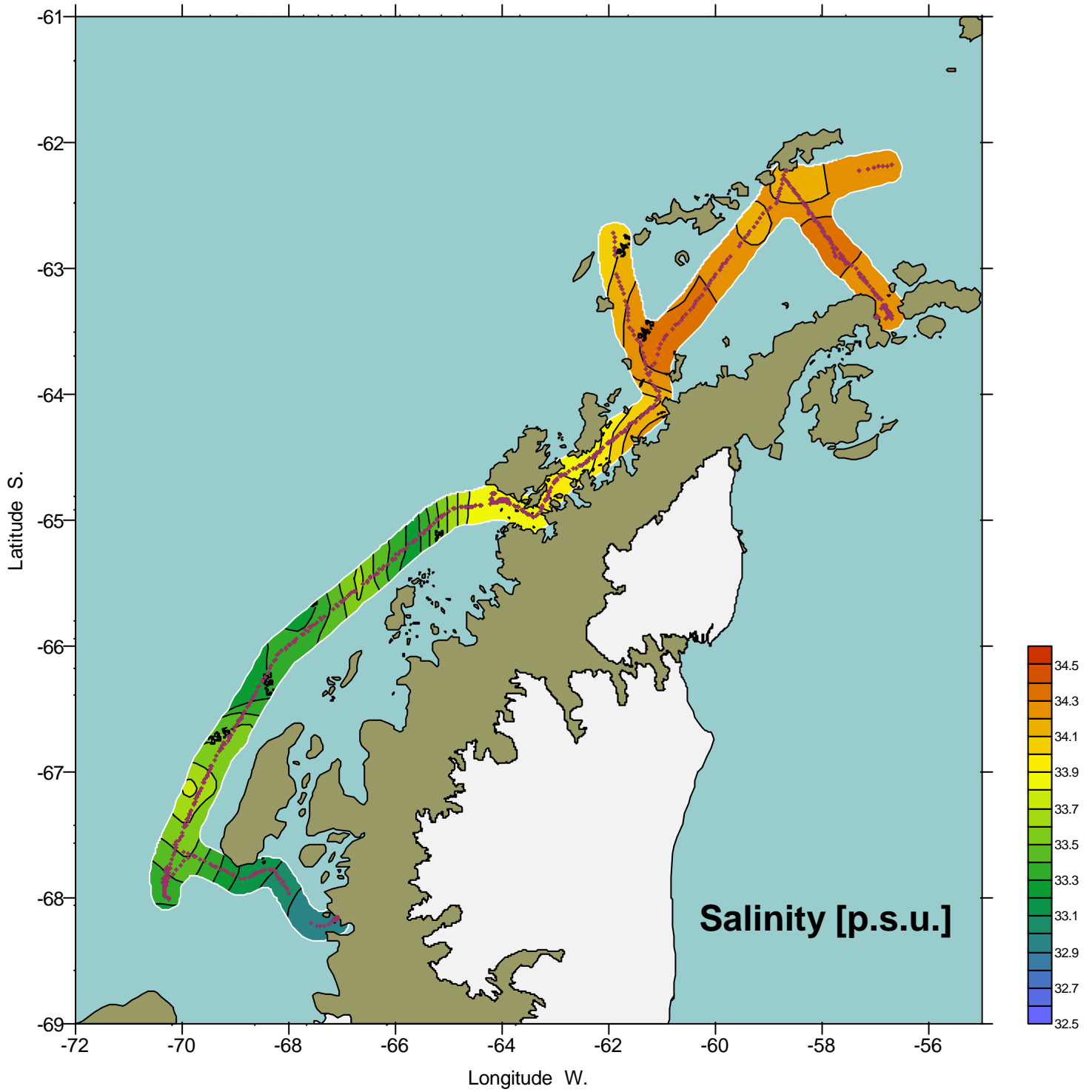
Sea-surface salinity distribution (April 2002)
