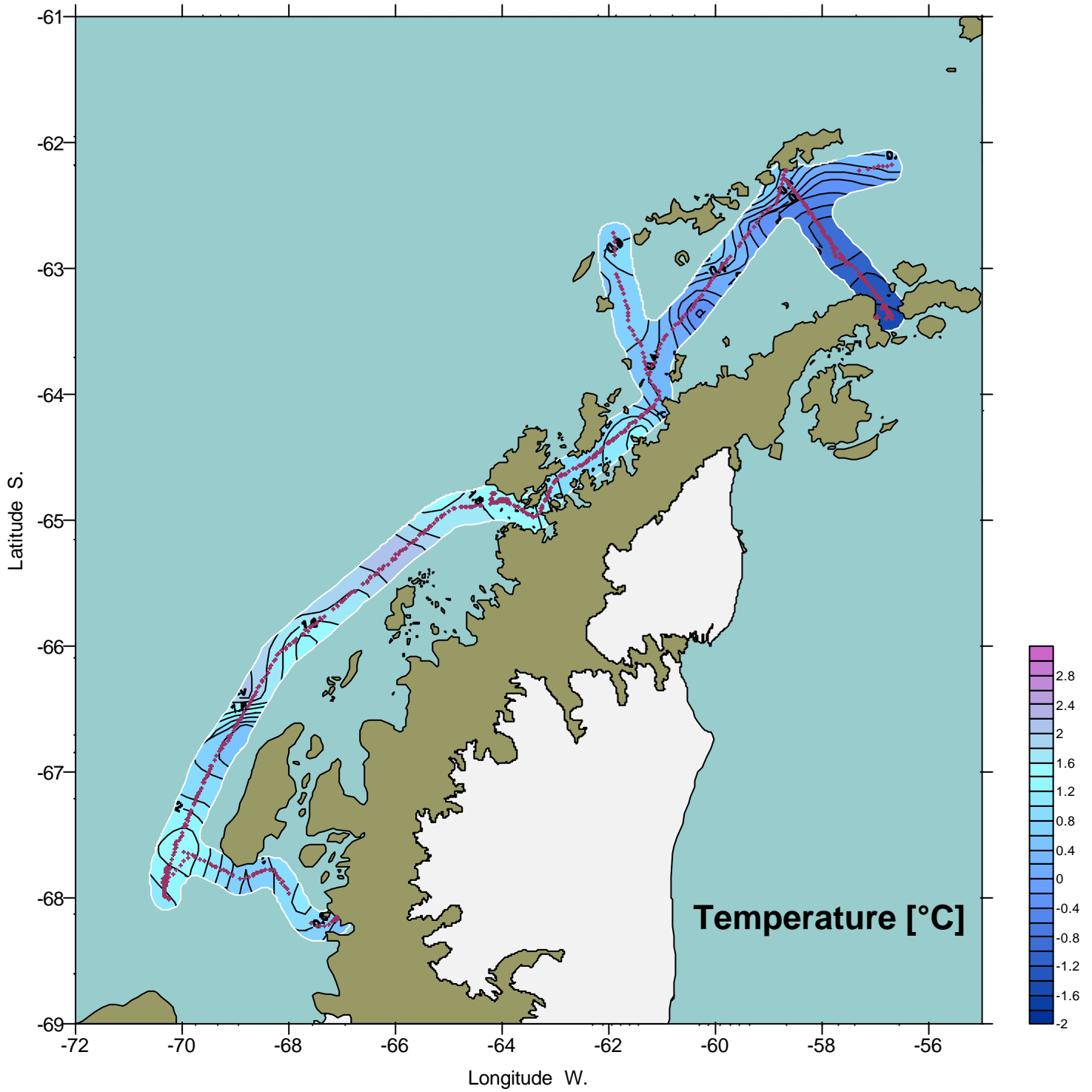
Sea-surface temperature distribution (April 2002)
