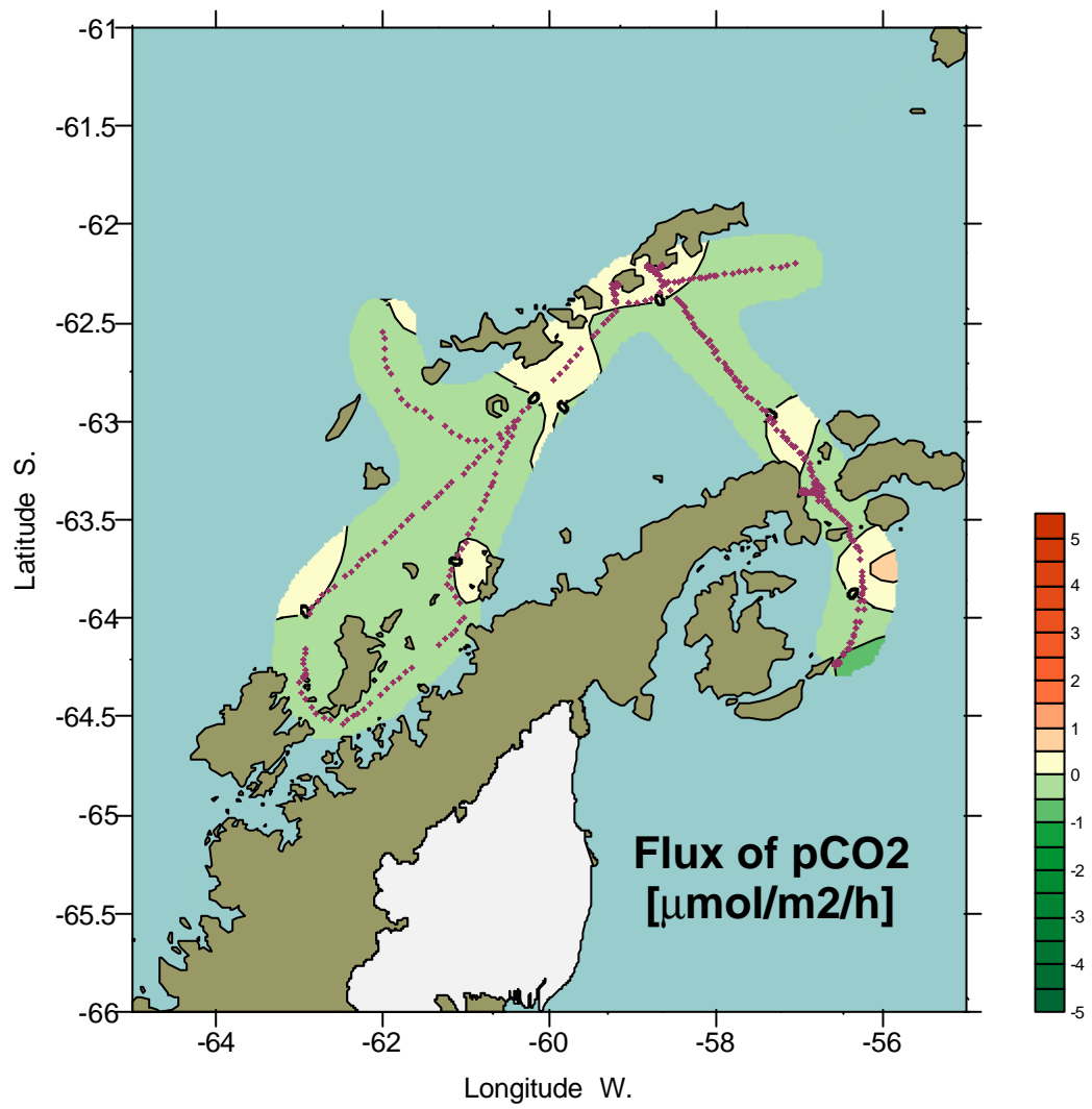
Flux of pCO 2 to atmosphere calculated by using measured wind (March 2002)
